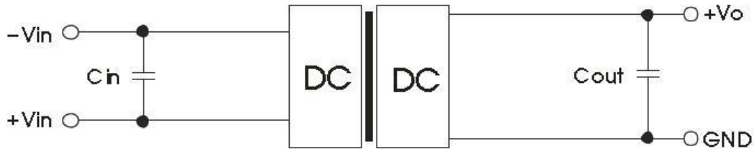
Note 1: C_{in} is 4.7uF/50V, C_{out} is 10uF/50V
